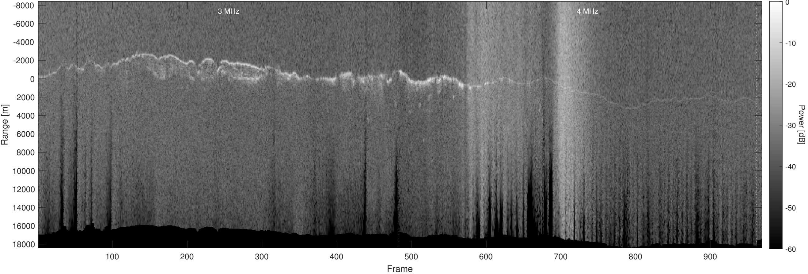
Orbit 12710, Optimized, Window, Depth-Corrected, Channel 2
