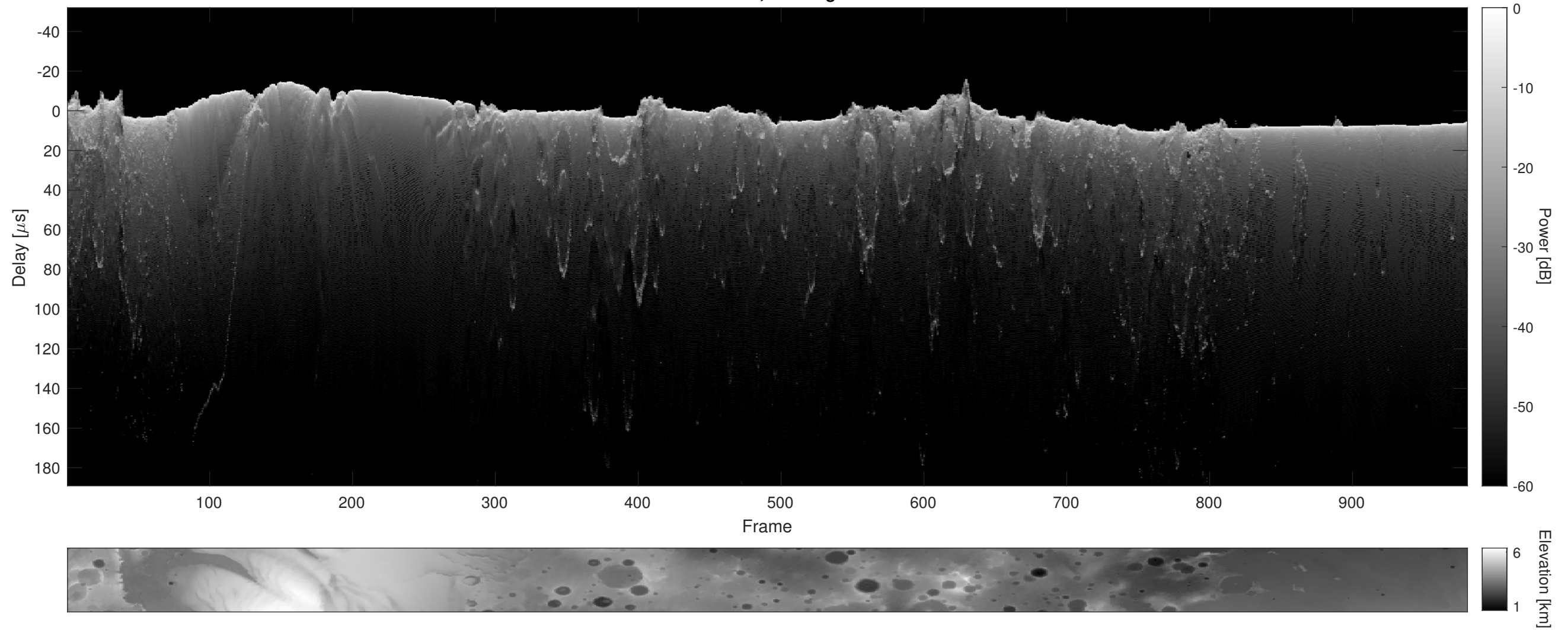
Orbit 12713, Cluttergram
