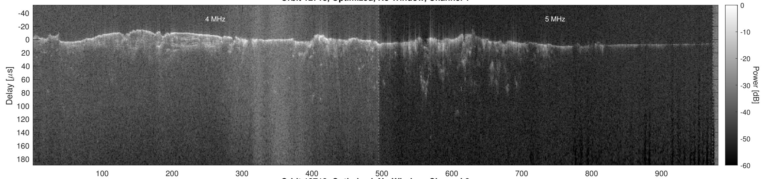
Orbit 12713, Optimized, No Window, Channel 2
