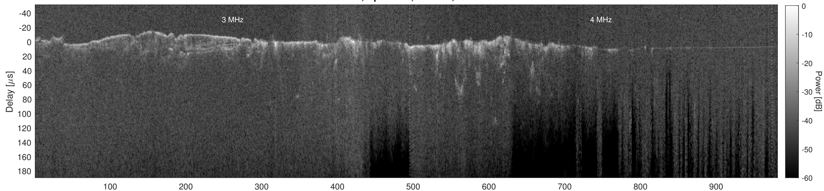
Orbit 12713, Cluttergram
