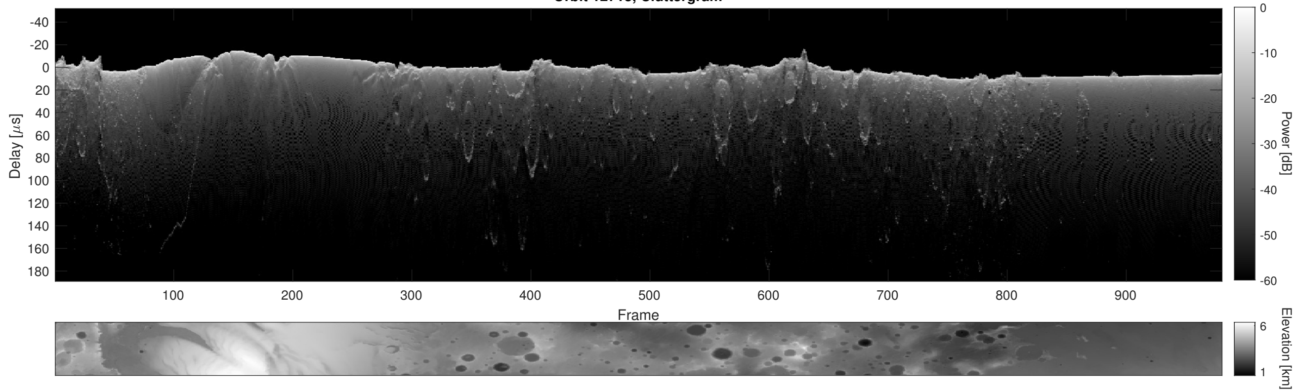
Orbit 12713, Cluttergram
