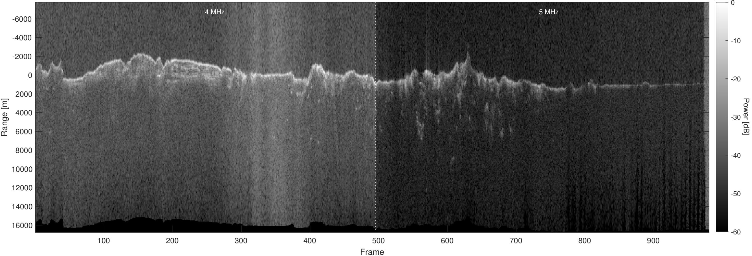
Orbit 12713, Optimized, Window, Depth-Corrected, Channel 2
