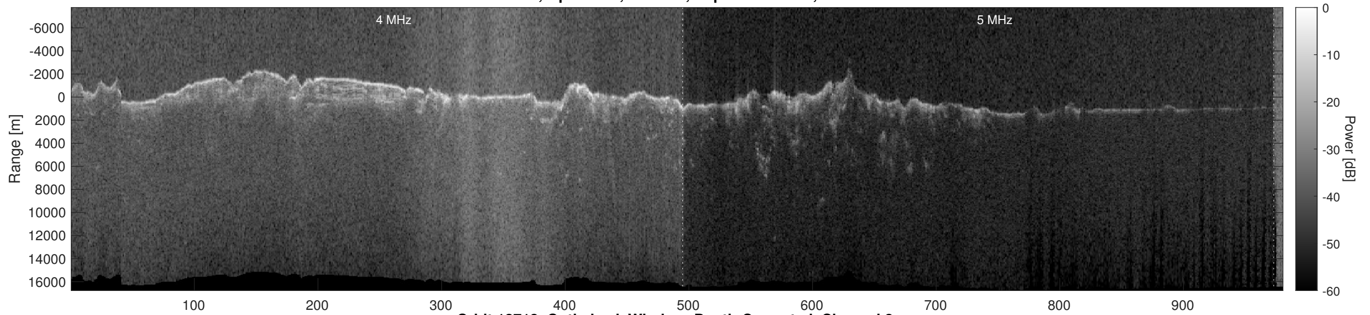
Orbit 12713, Optimized, Window, Depth-Corrected, Channel 2
