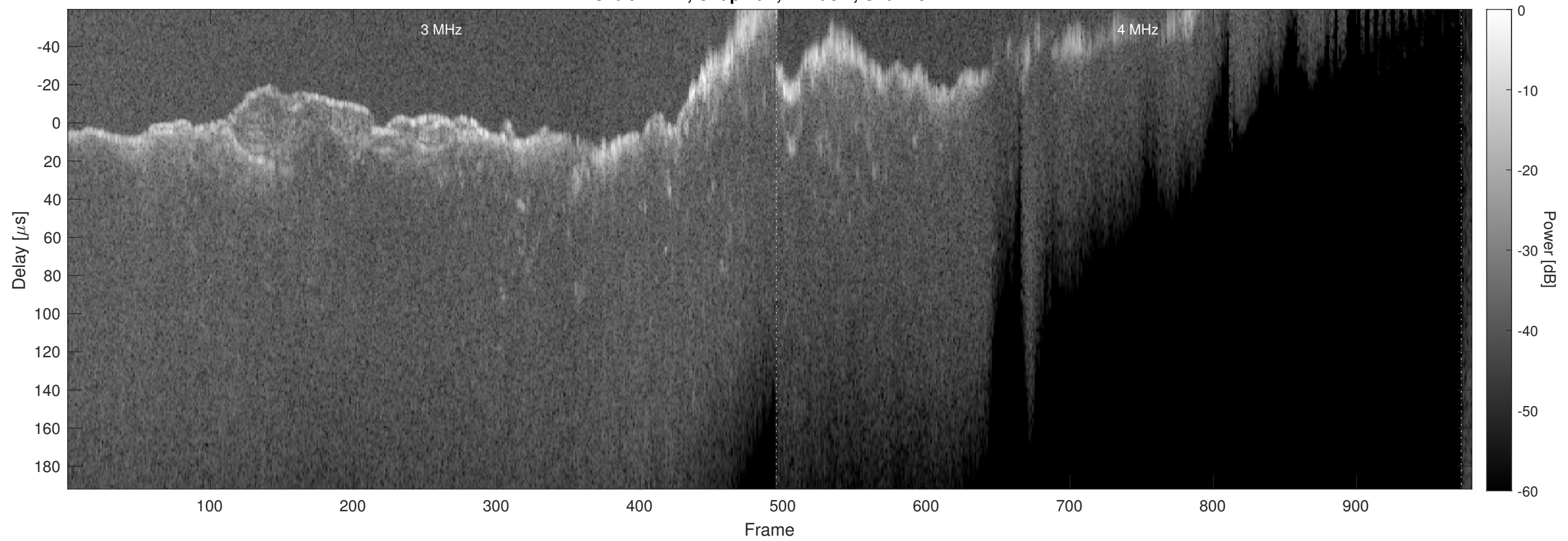
Orbit 12714, Chapman, Window, Channel 2
