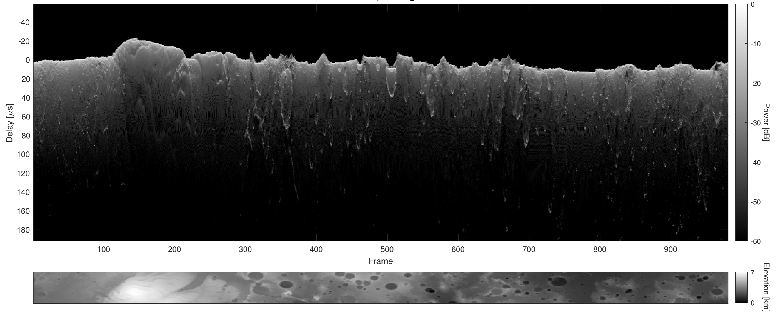
Orbit 12714, Cluttergram
