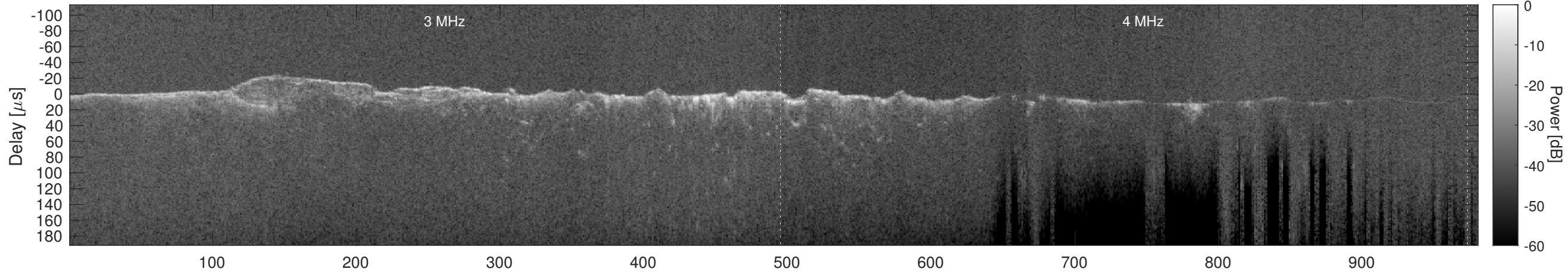
Orbit 12714, Cluttergram
