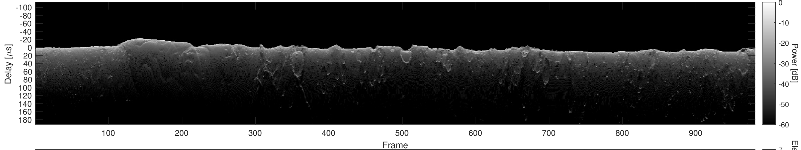
Orbit 12714, Cluttergram
