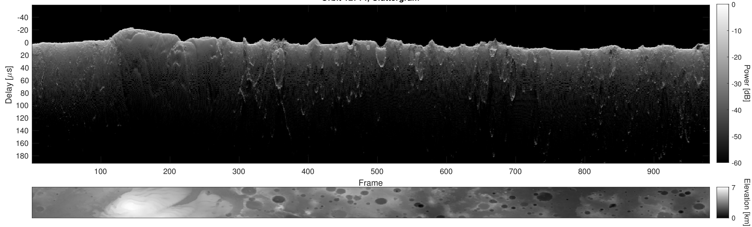
Orbit 12714, Cluttergram
