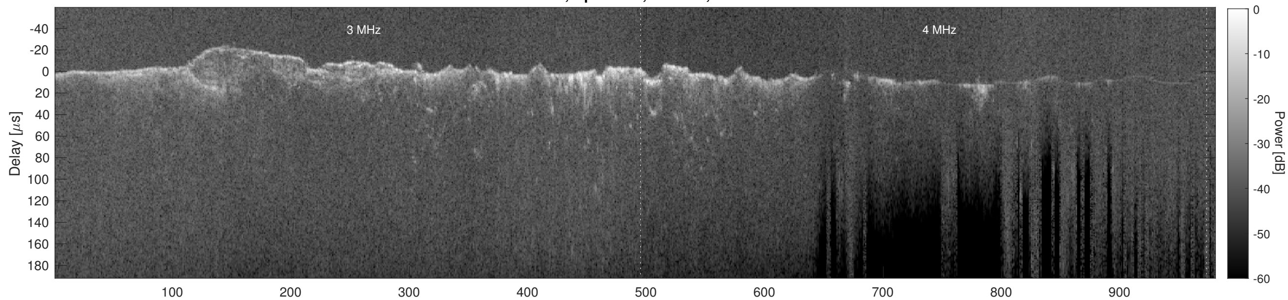
Orbit 12714, Cluttergram
