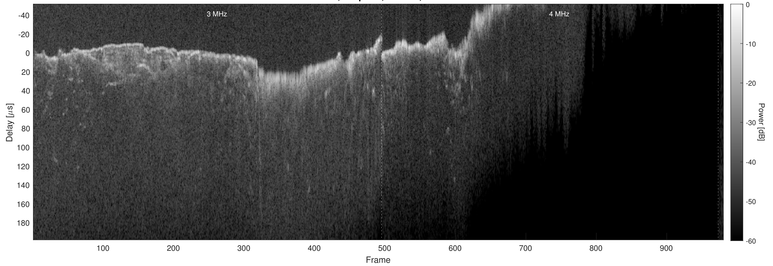
Orbit 12716, Chapman, Window, Channel 2
