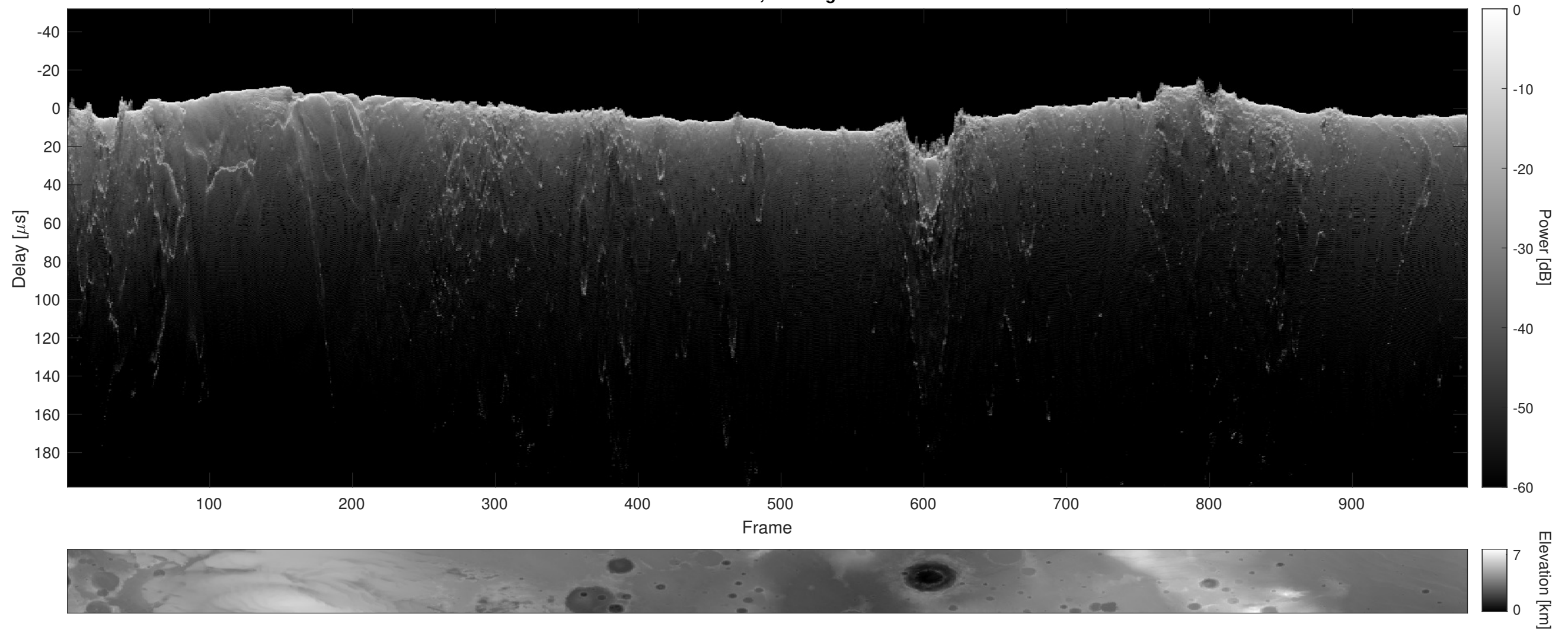
Orbit 12716, Cluttergram
