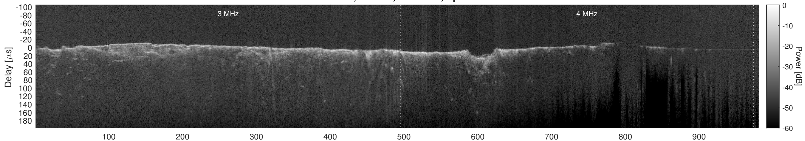
Orbit 12716, Cluttergram
