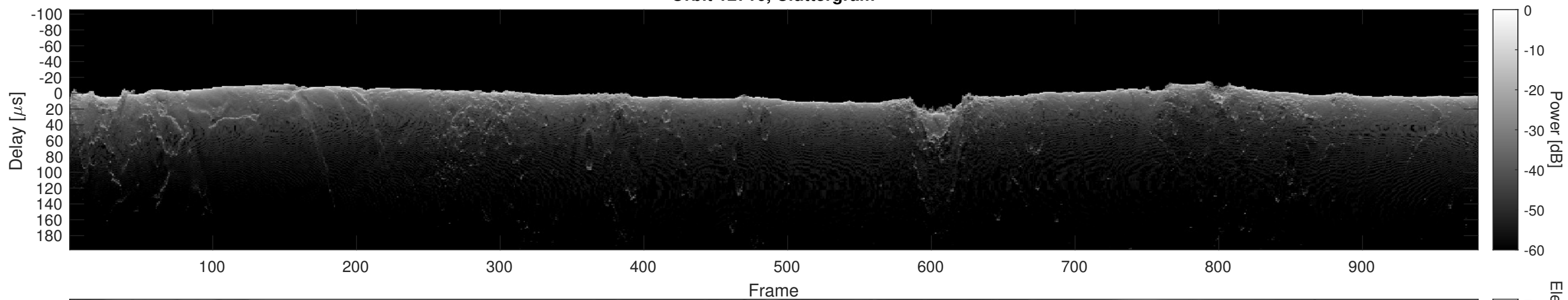
Orbit 12716, Cluttergram
