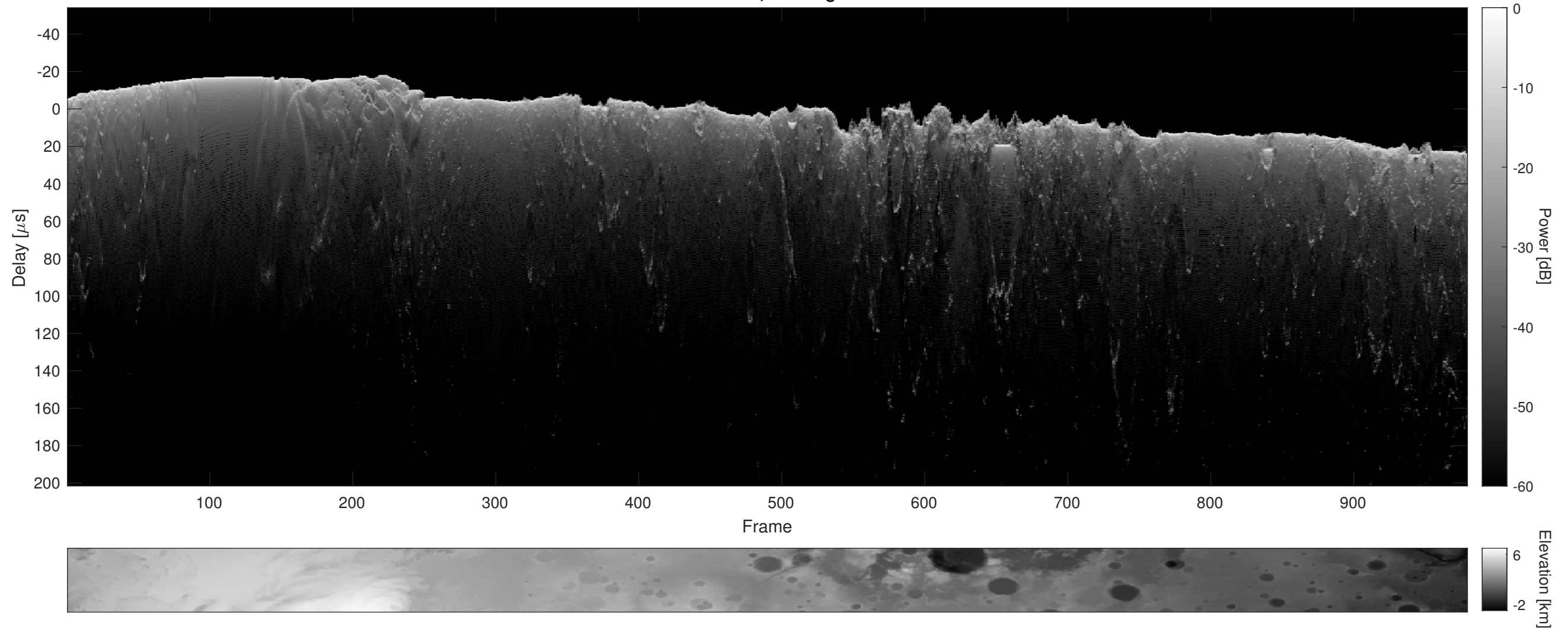
Orbit 12719, Cluttergram
