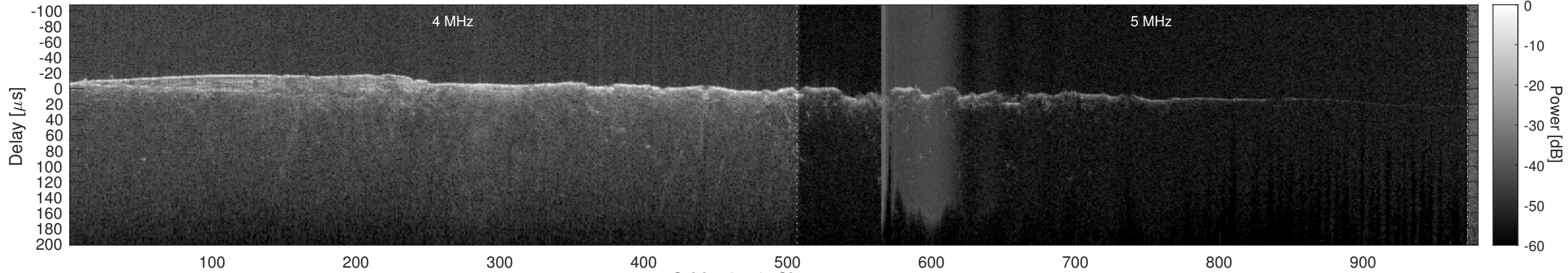
Orbit 12719, Cluttergram
