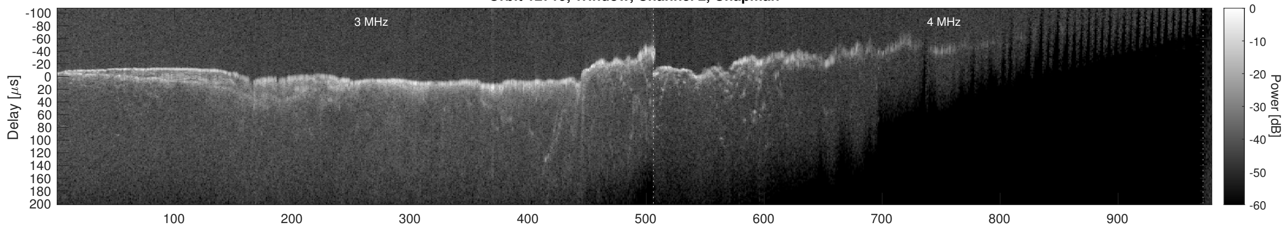
Orbit 12719, Window, Channel 2, Optimized
