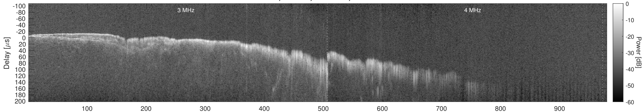
Orbit 12719, Window, Channel 2, Chapman
