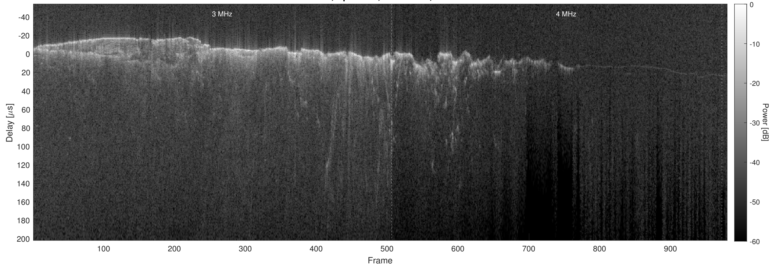
Orbit 12719, Optimized, No Window, Channel 2
