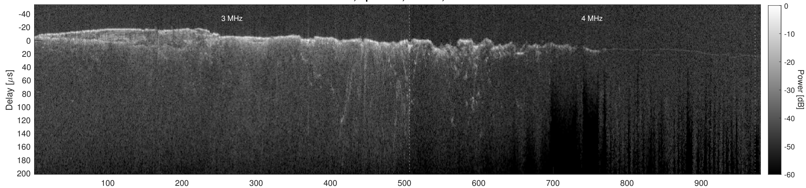
Orbit 12719, Cluttergram
