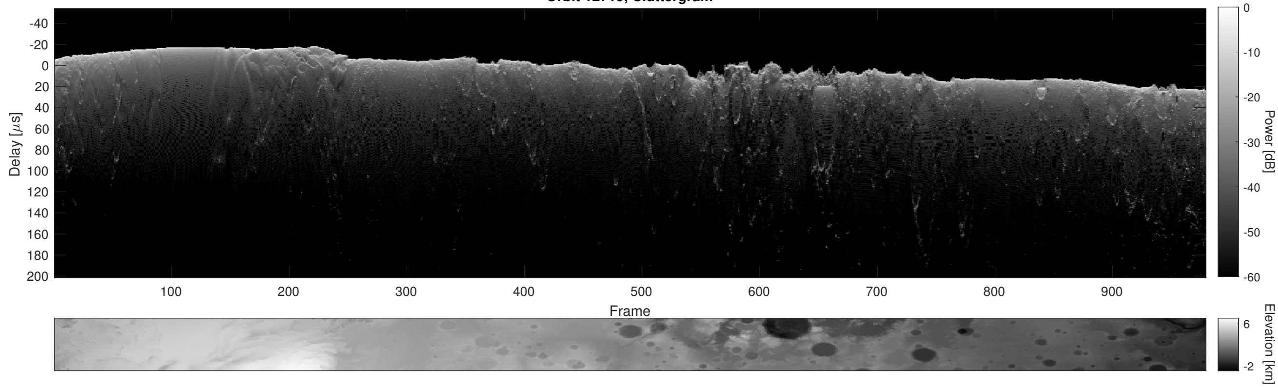
Orbit 12719, Cluttergram
