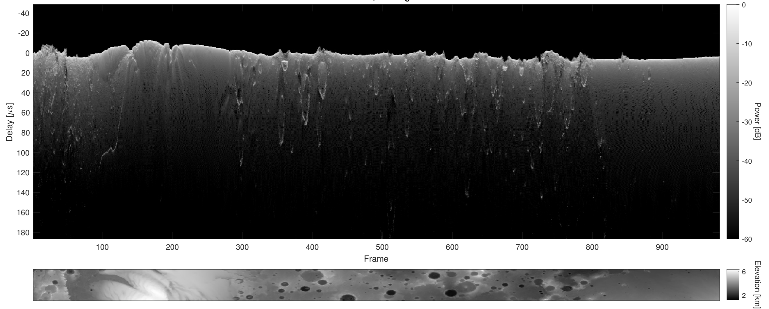
Orbit 12720, Cluttergram
