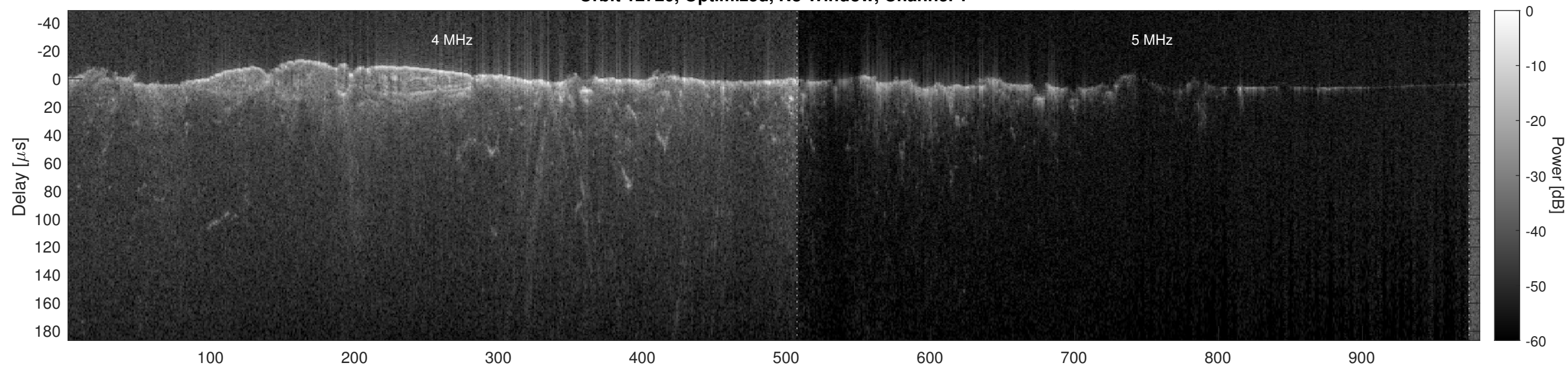
Orbit 12720, Optimized, No Window, Channel 2
