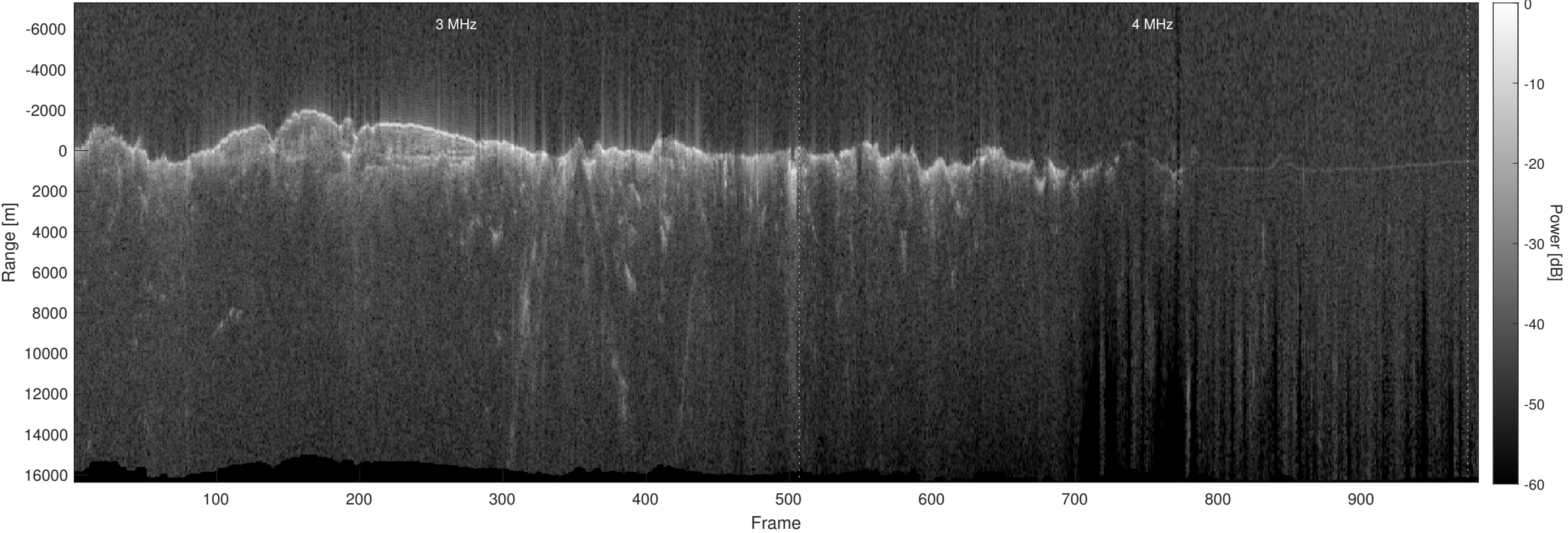
Orbit 12720, Optimized, No Window, Depth-Corrected, Channel 2
