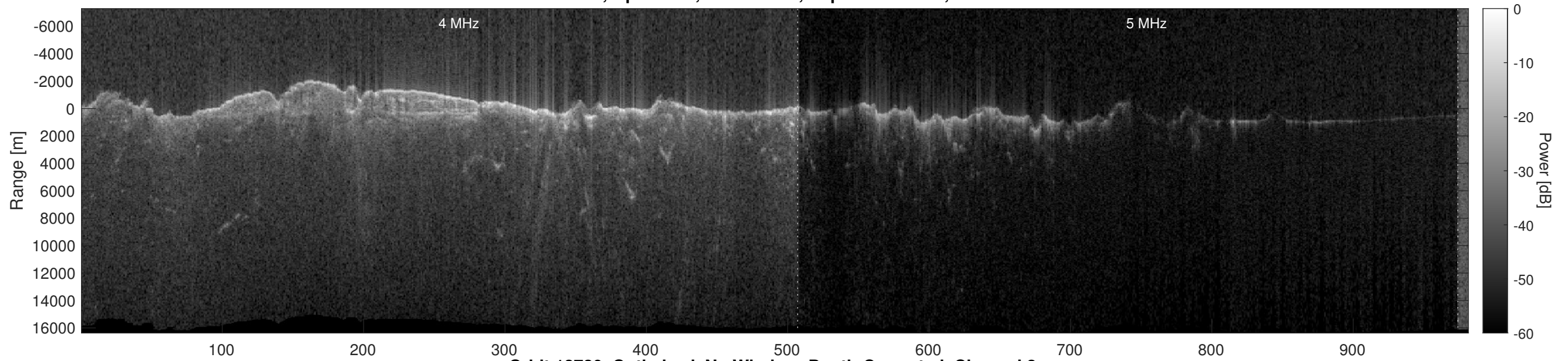
Orbit 12720, Optimized, No Window, Depth-Corrected, Channel 2
