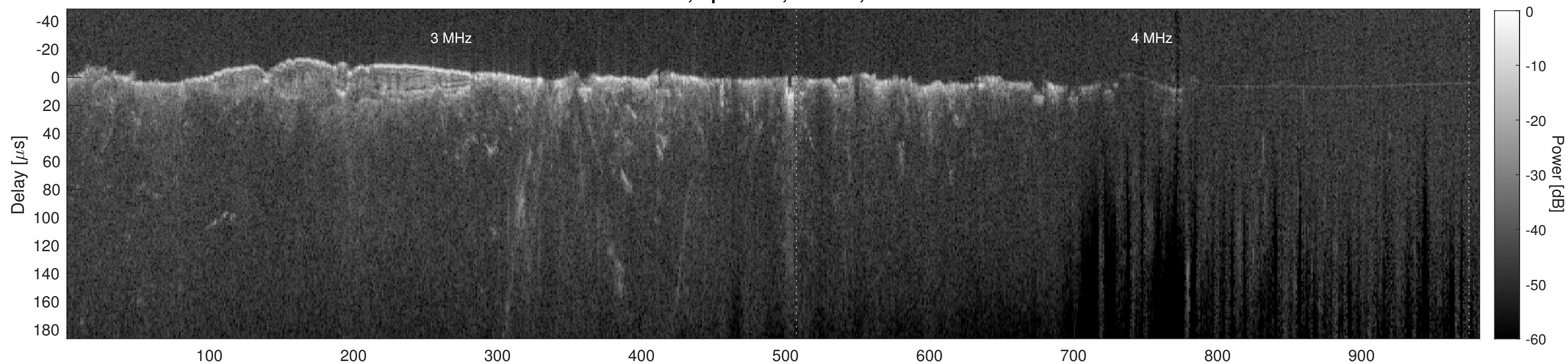
Orbit 12720, Cluttergram
