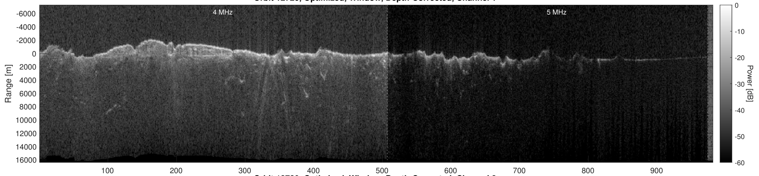
Orbit 12720, Optimized, Window, Depth-Corrected, Channel 2
