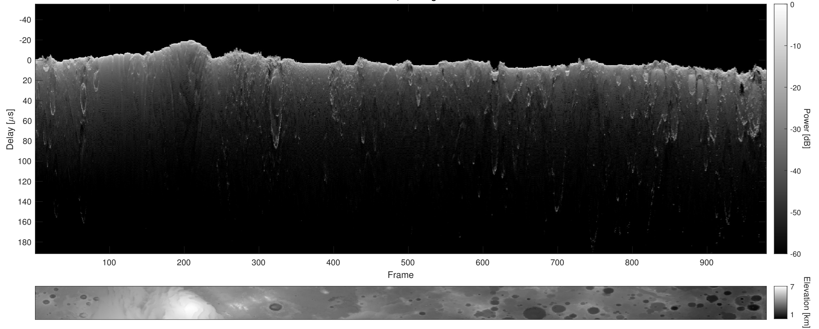
Orbit 12722, Cluttergram
