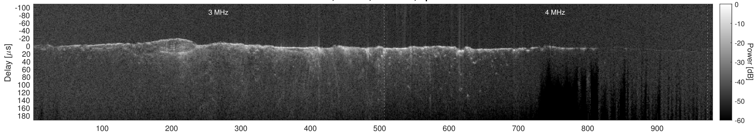
Orbit 12722, Cluttergram
