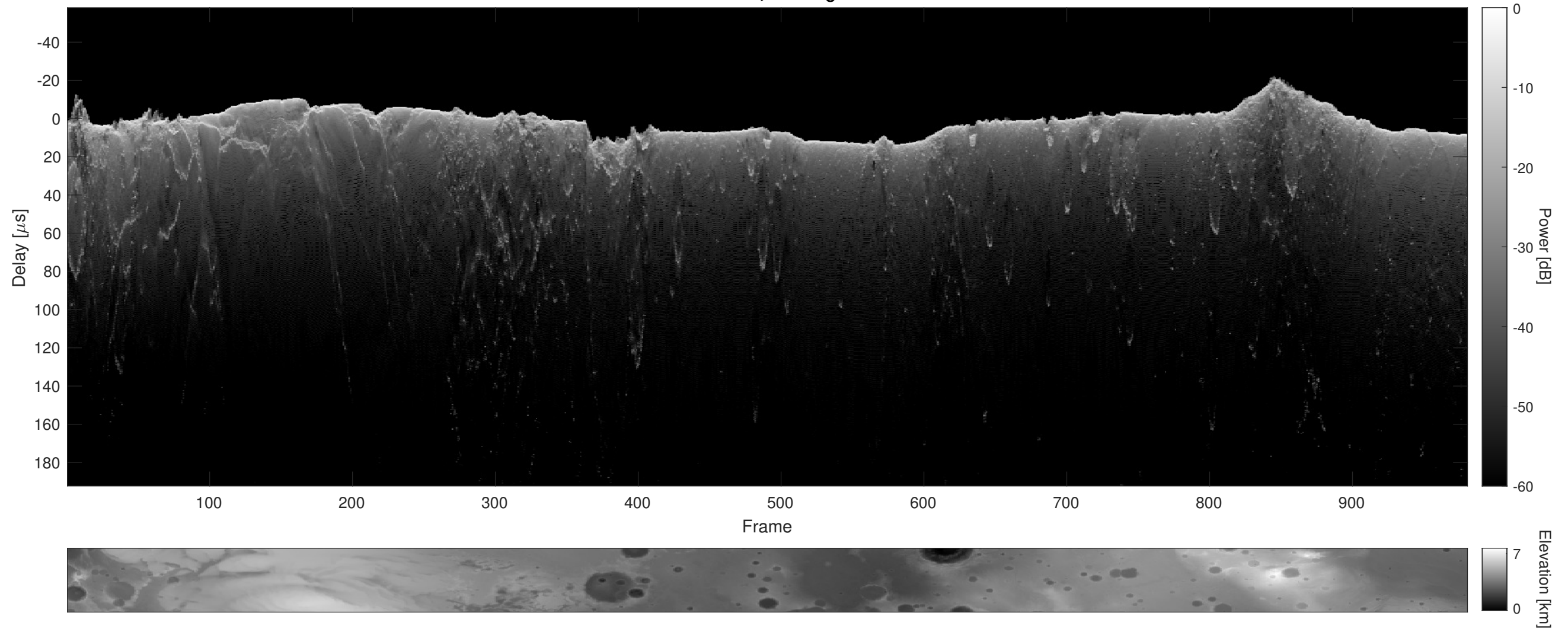
Orbit 12723, Cluttergram
