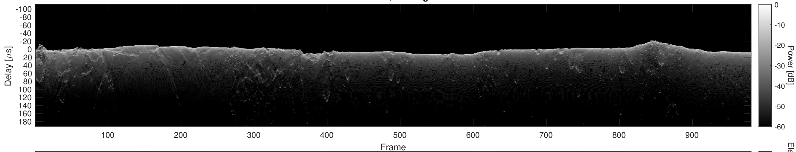
Orbit 12723, Cluttergram
