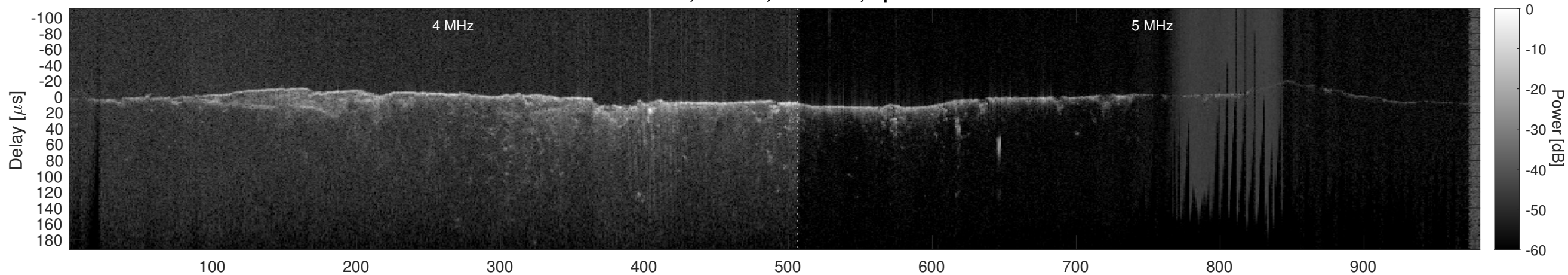
Orbit 12723, Cluttergram
