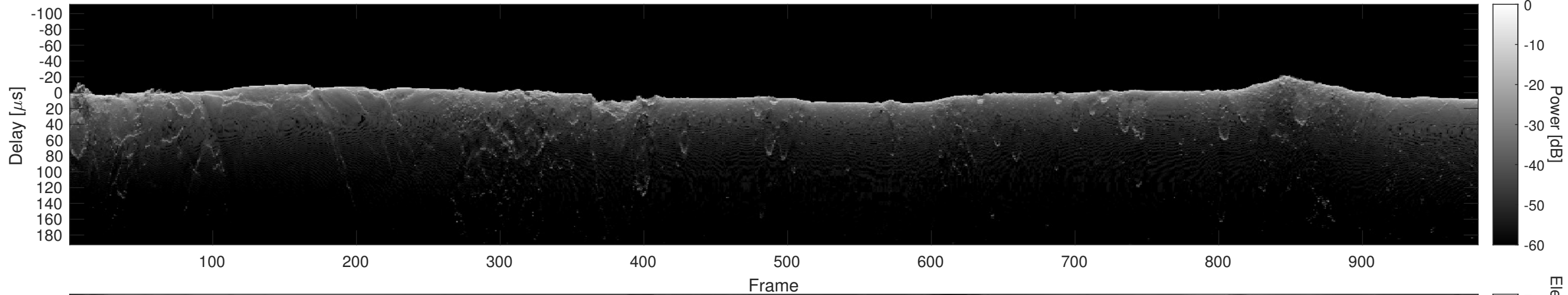
Orbit 12723, Cluttergram
