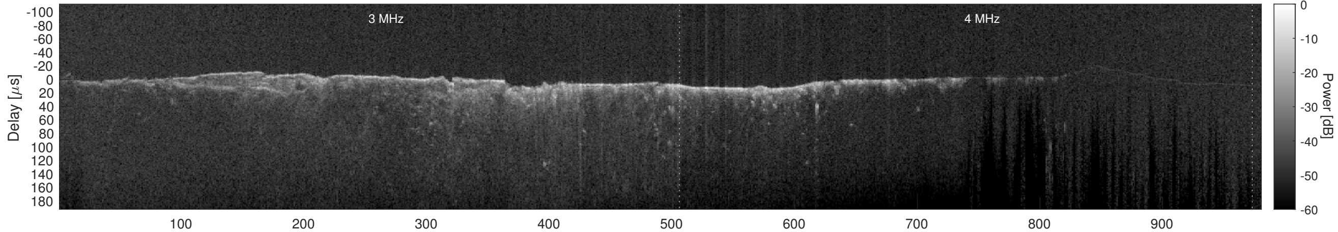
Orbit 12723, Cluttergram
