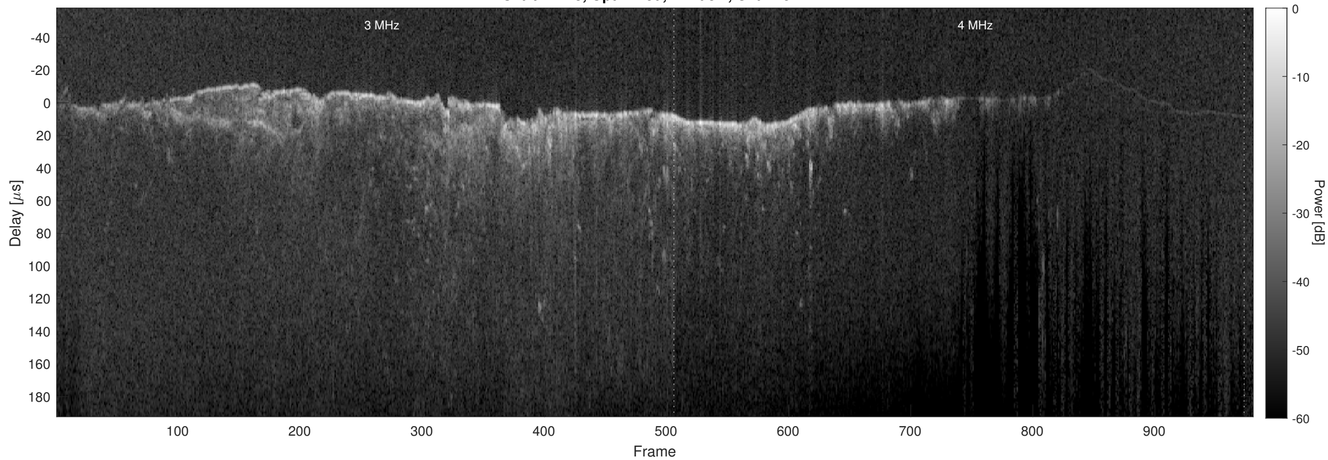
Orbit 12723, Optimized, Window, Channel 2
