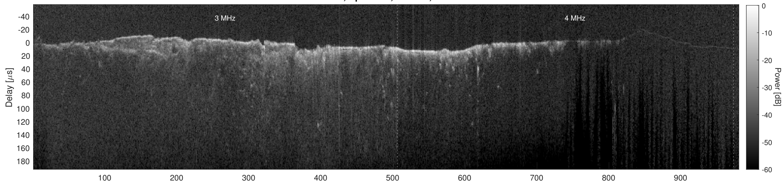
Orbit 12723, Cluttergram
