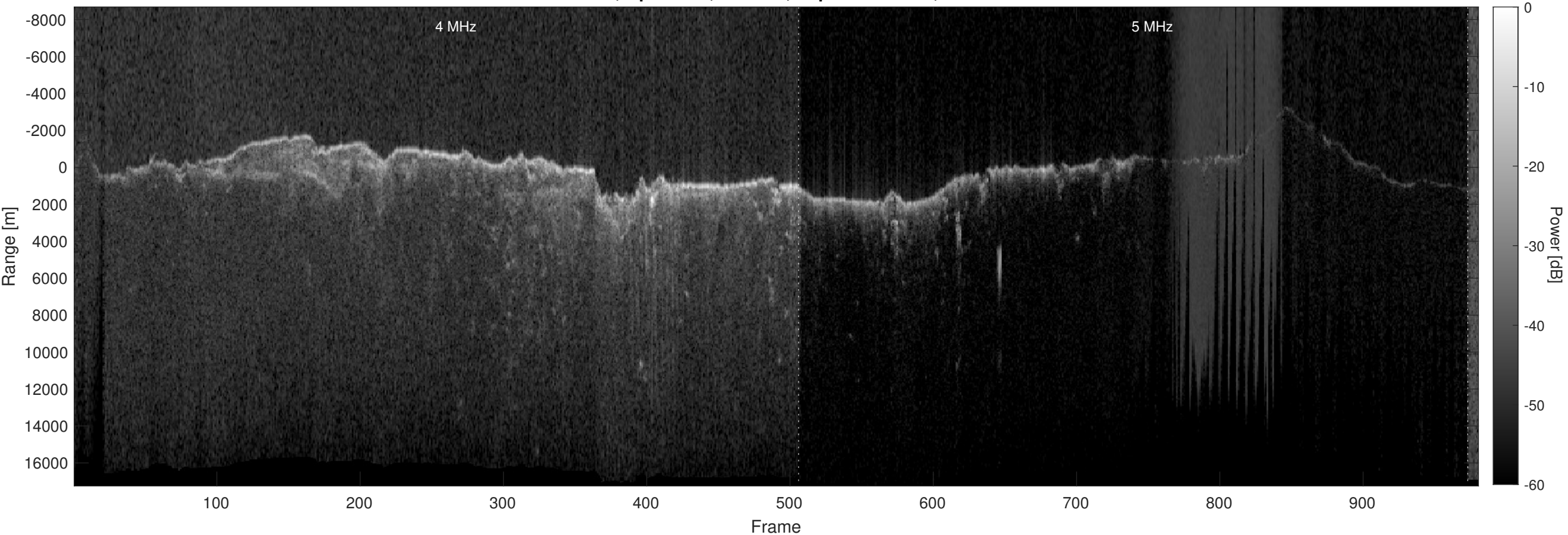
Orbit 12723, Optimized, Window, Depth-Corrected, Channel 2
