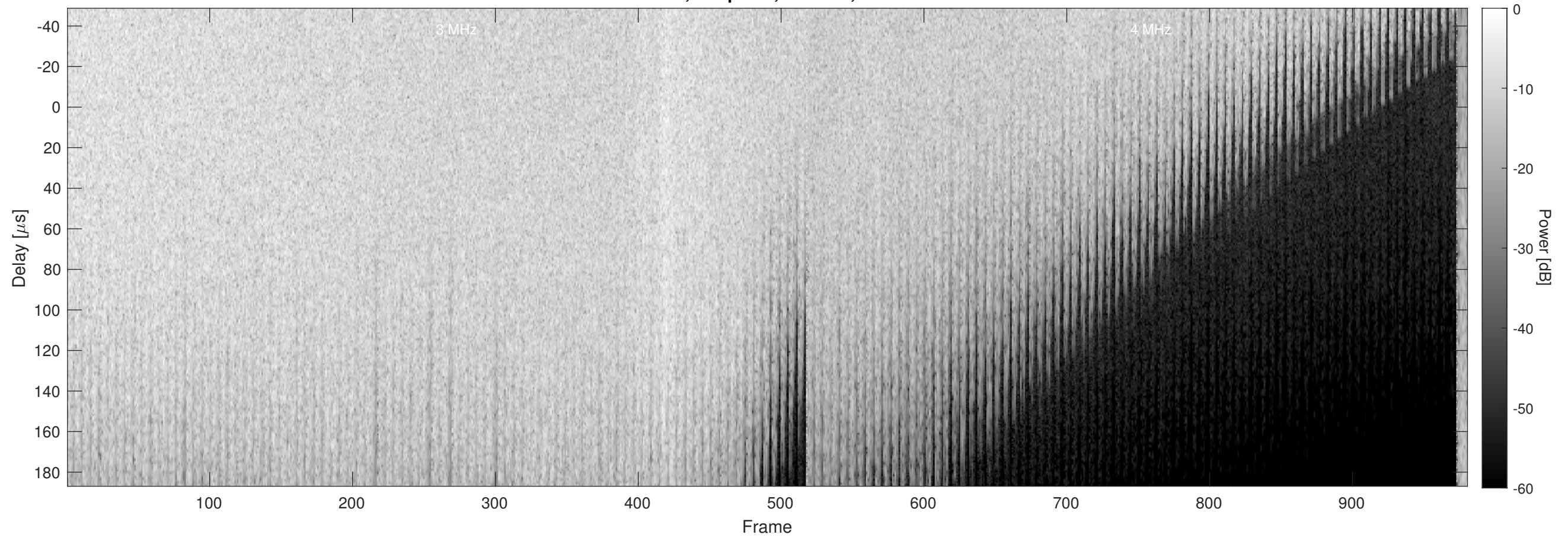
Orbit 12727, Chapman, Window, Channel 2
