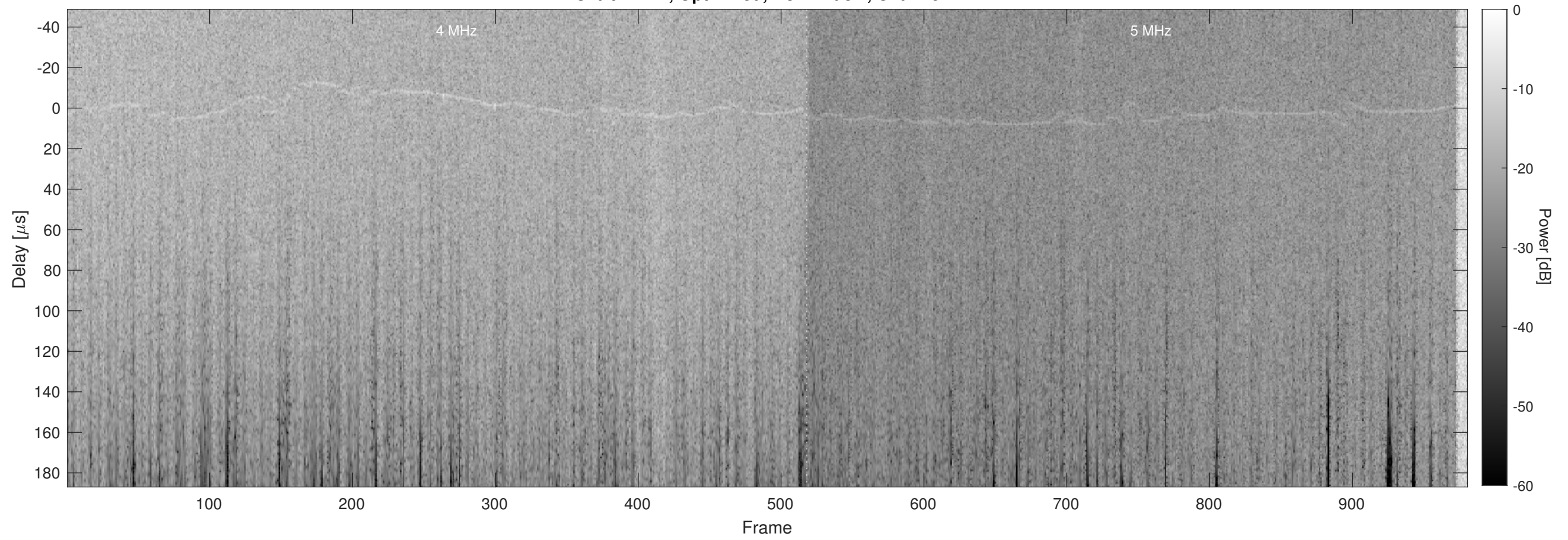
Orbit 12727, Optimized, No Window, Channel 2
