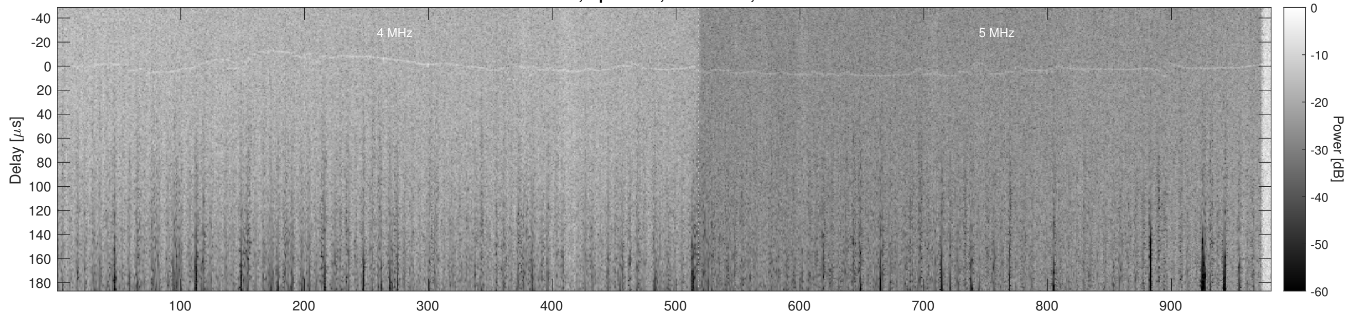
Orbit 12727, Optimized, No Window, Channel 2
