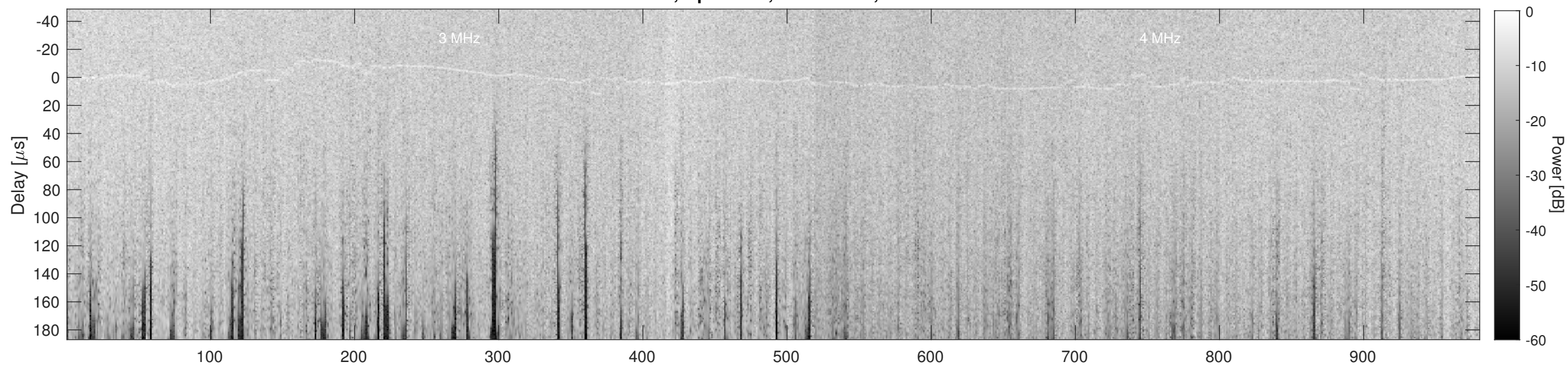
Orbit 12727, Cluttergram
