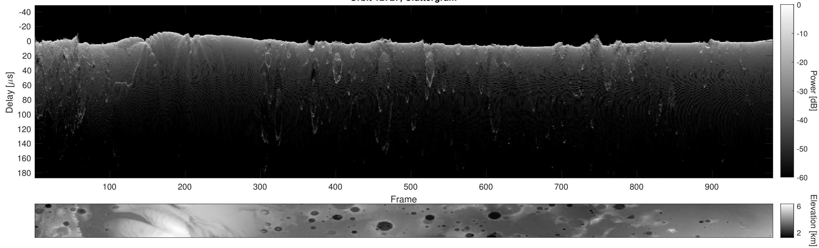
Orbit 12727, Cluttergram
