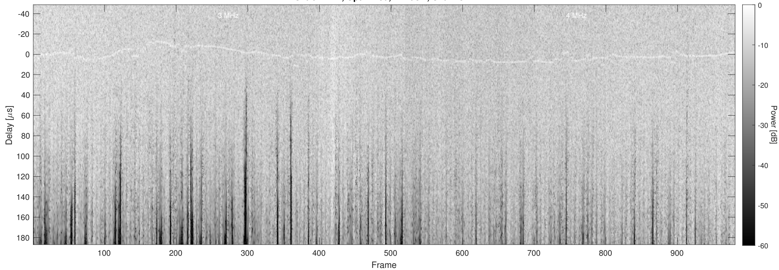
Orbit 12727, Optimized, Window, Channel 2
