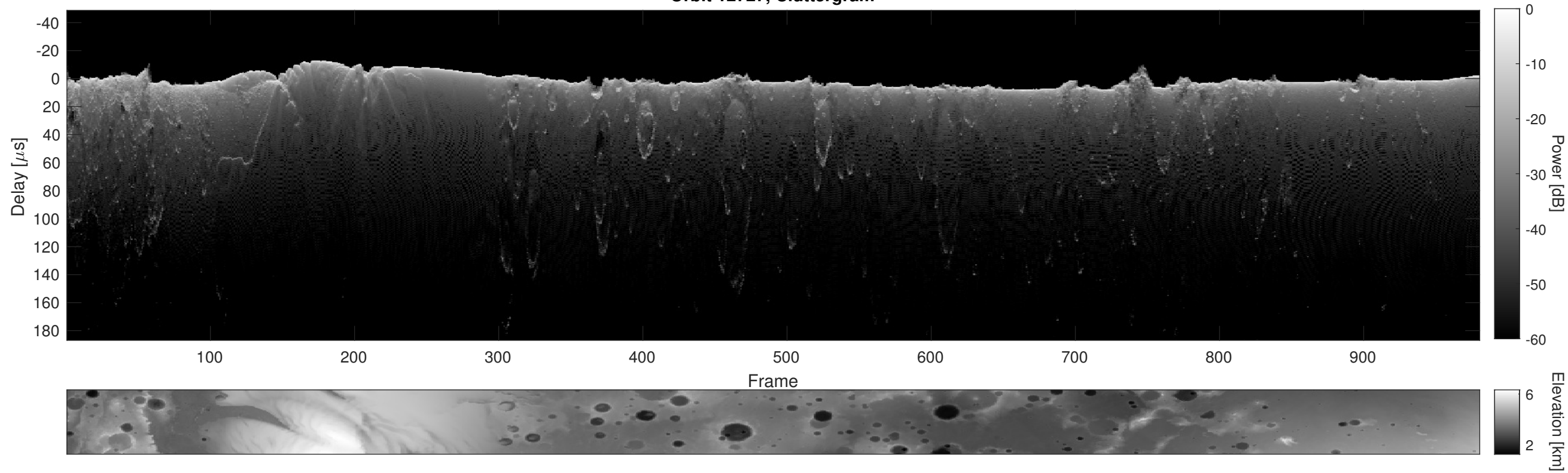
Orbit 12727, Cluttergram
