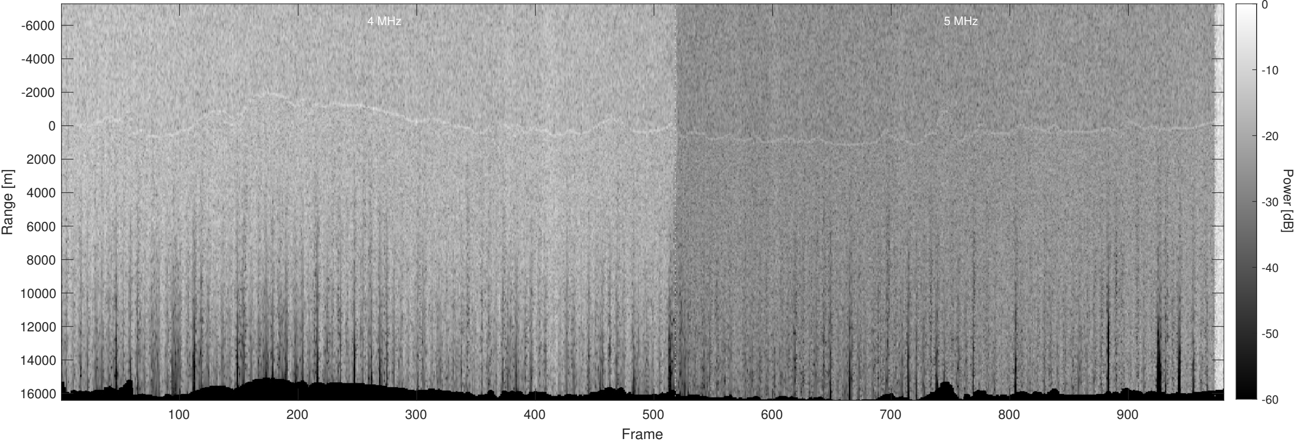
Orbit 12727, Optimized, Window, Depth-Corrected, Channel 2
