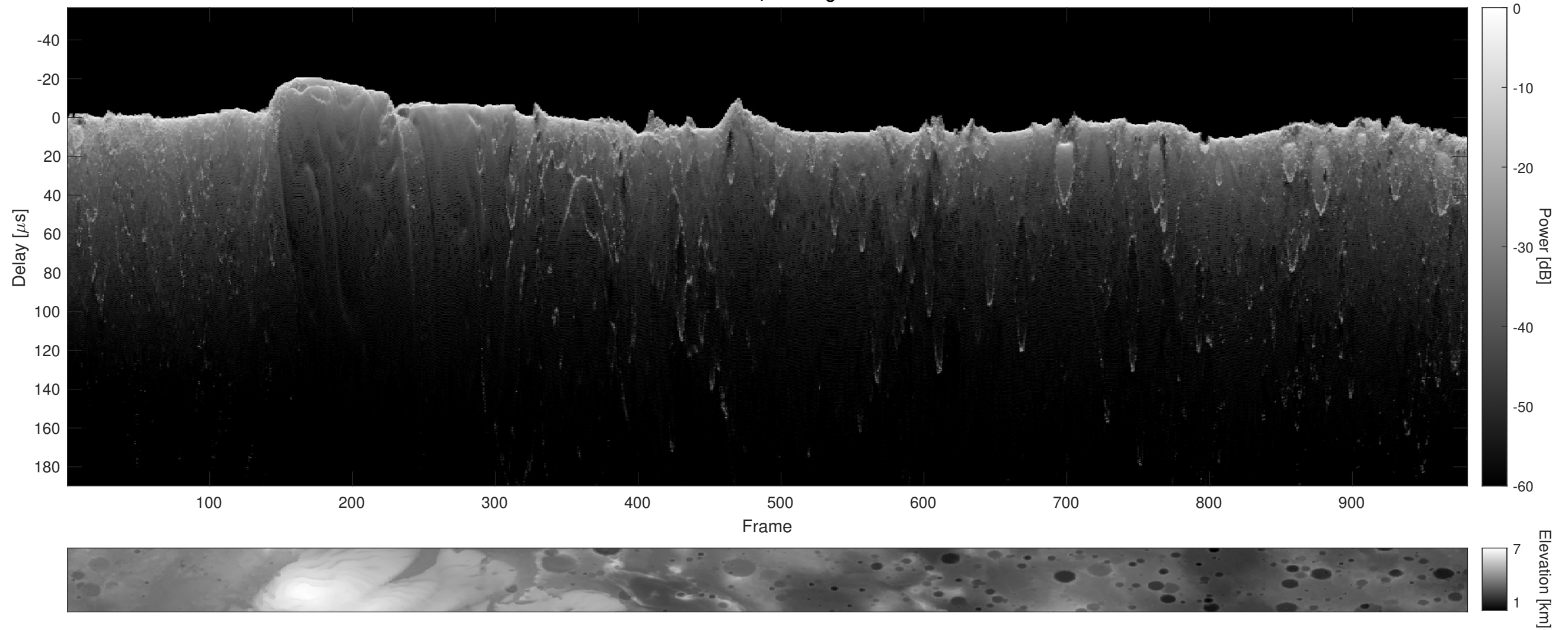
Orbit 12728, Cluttergram
