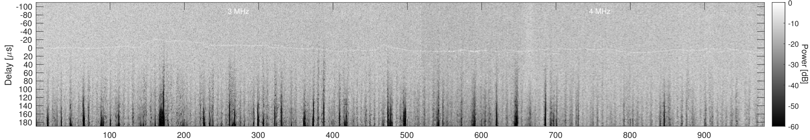
Orbit 12728, Cluttergram
