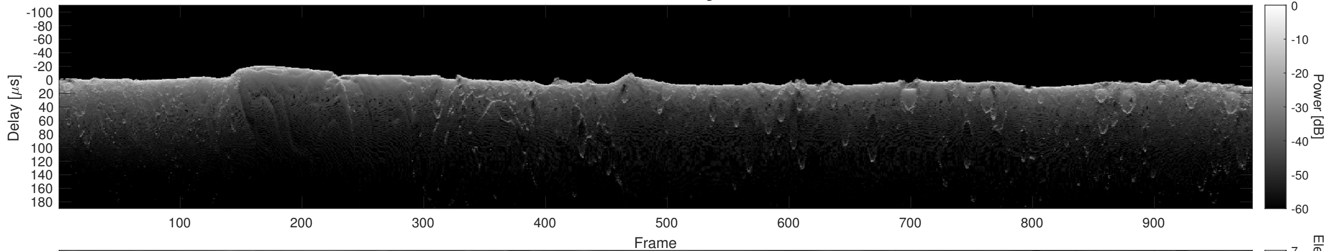
Orbit 12728, Cluttergram
