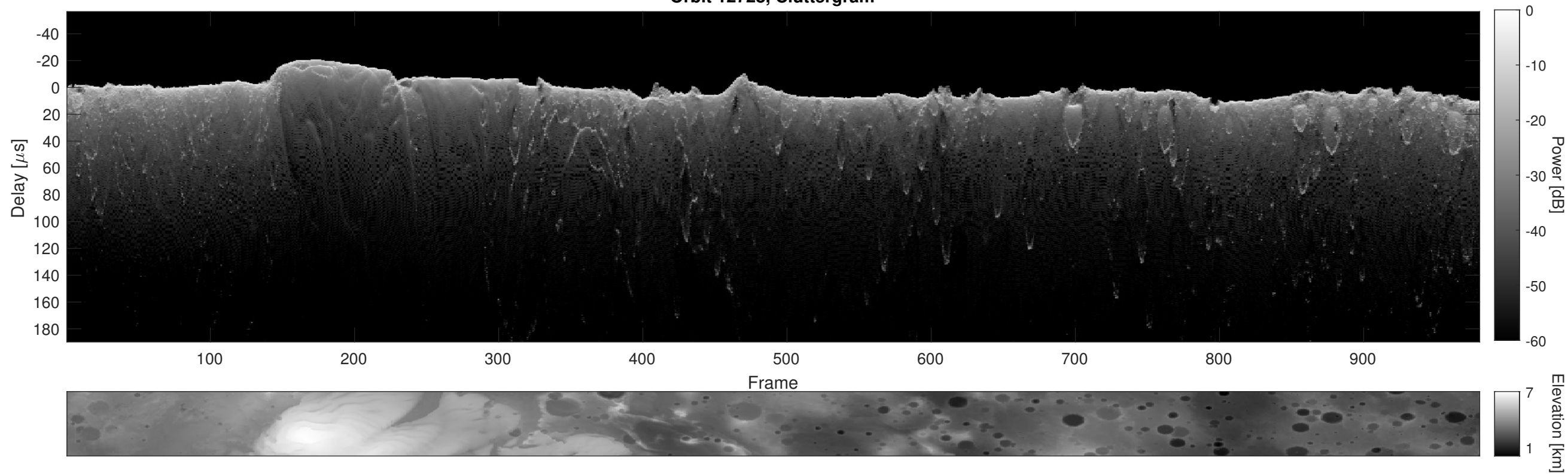
Orbit 12728, Cluttergram
