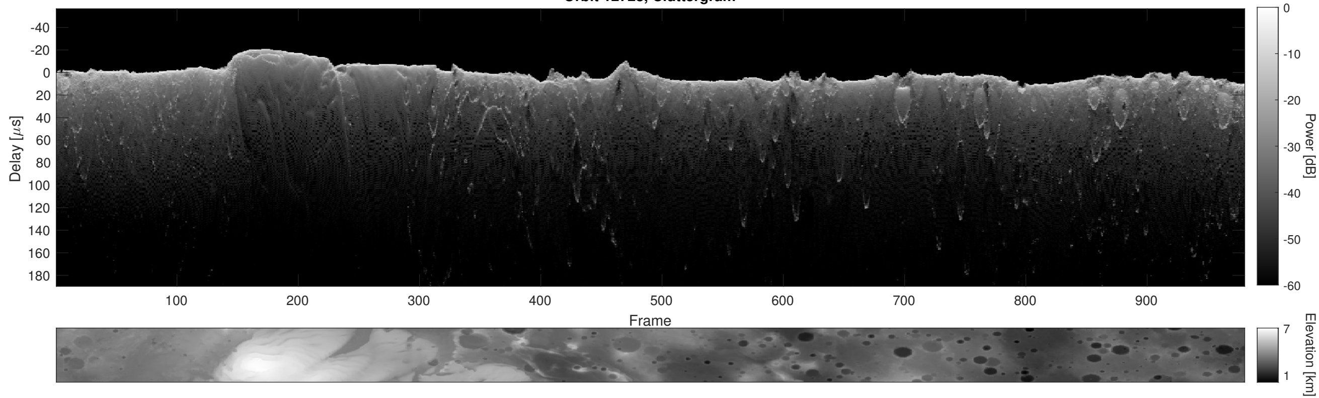
Orbit 12728, Cluttergram
