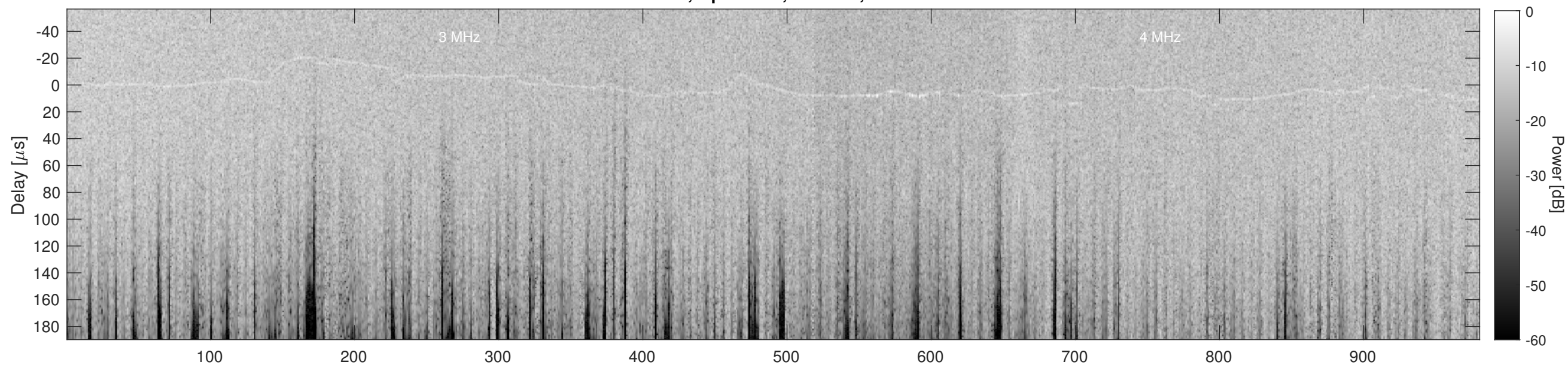
Orbit 12728, Cluttergram
