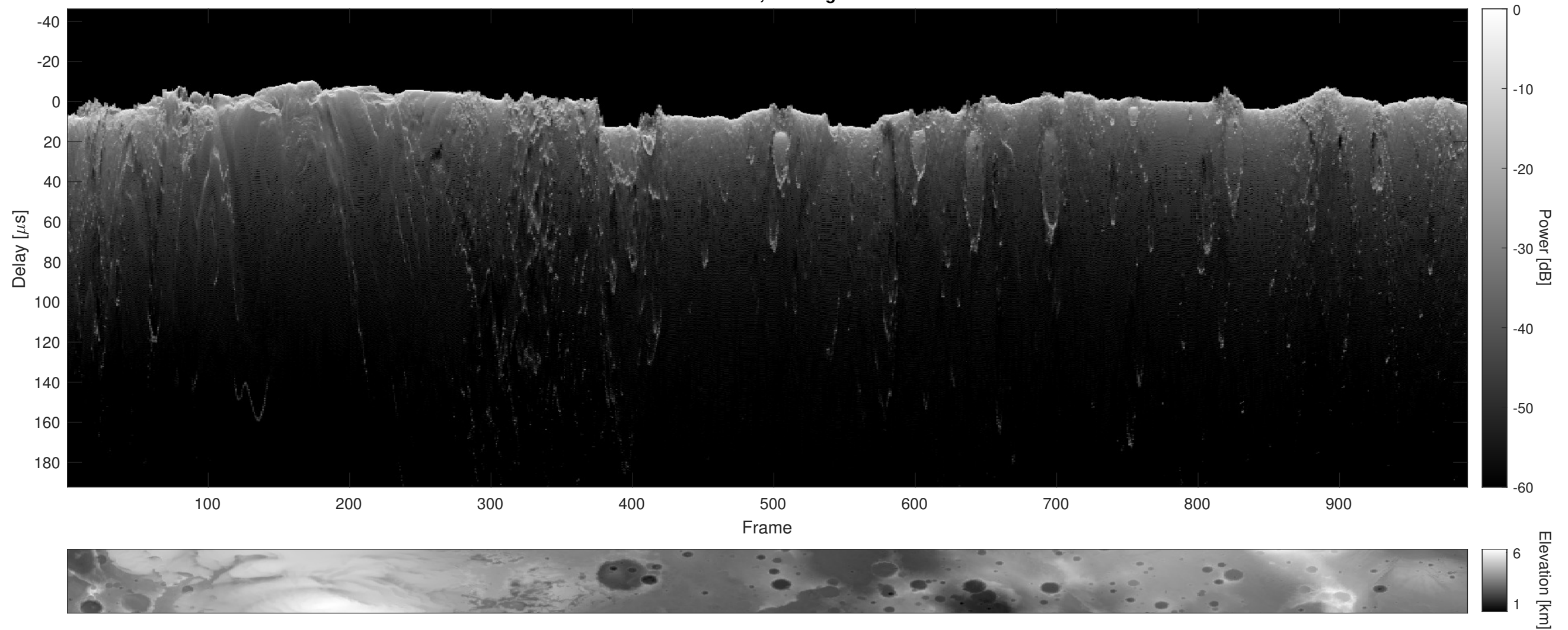
Orbit 12730, Cluttergram
