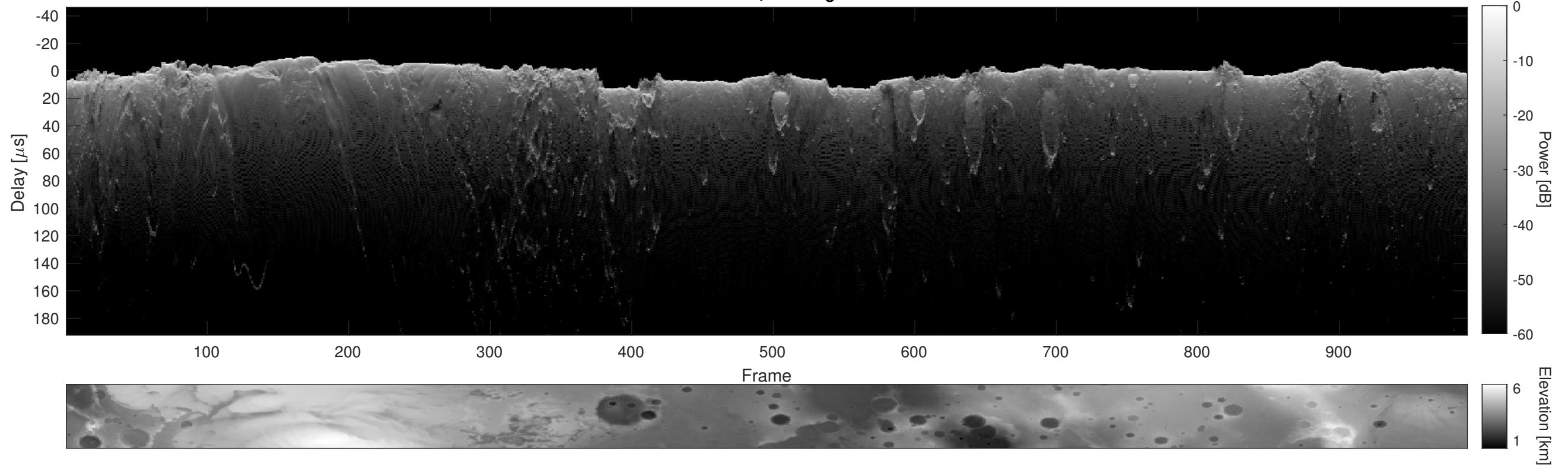
Orbit 12730, Cluttergram
