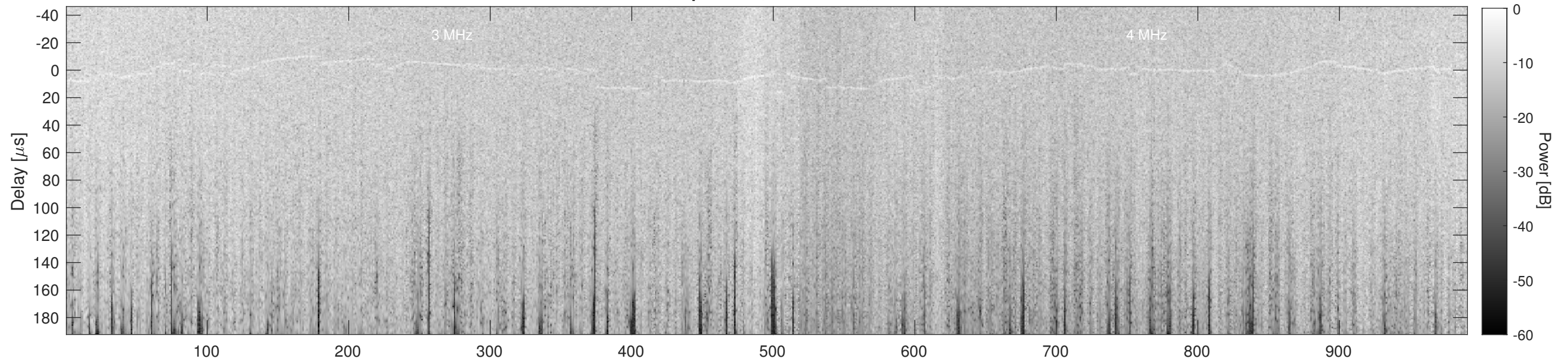
Orbit 12730, Cluttergram
