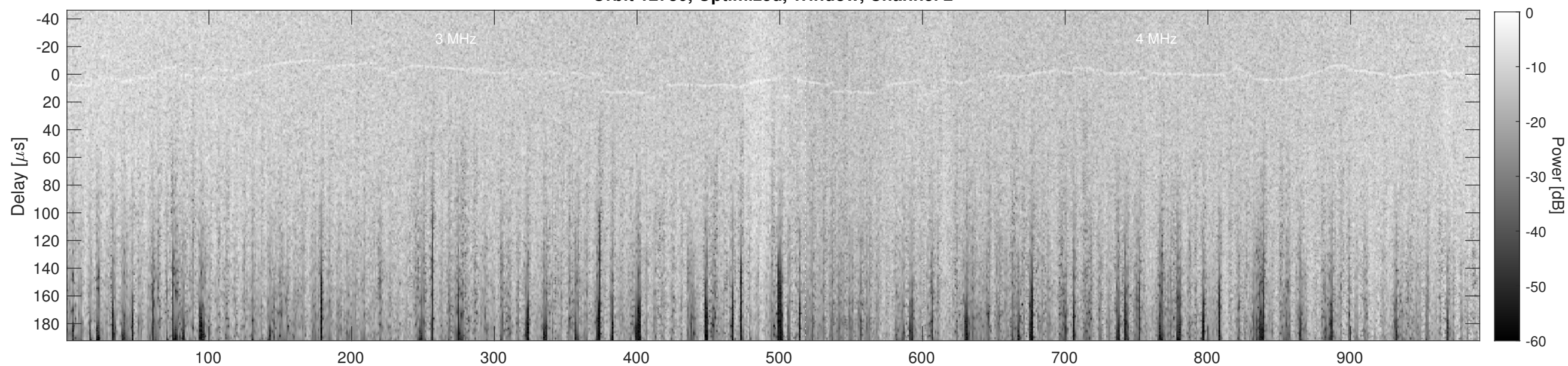
Orbit 12730, Cluttergram
