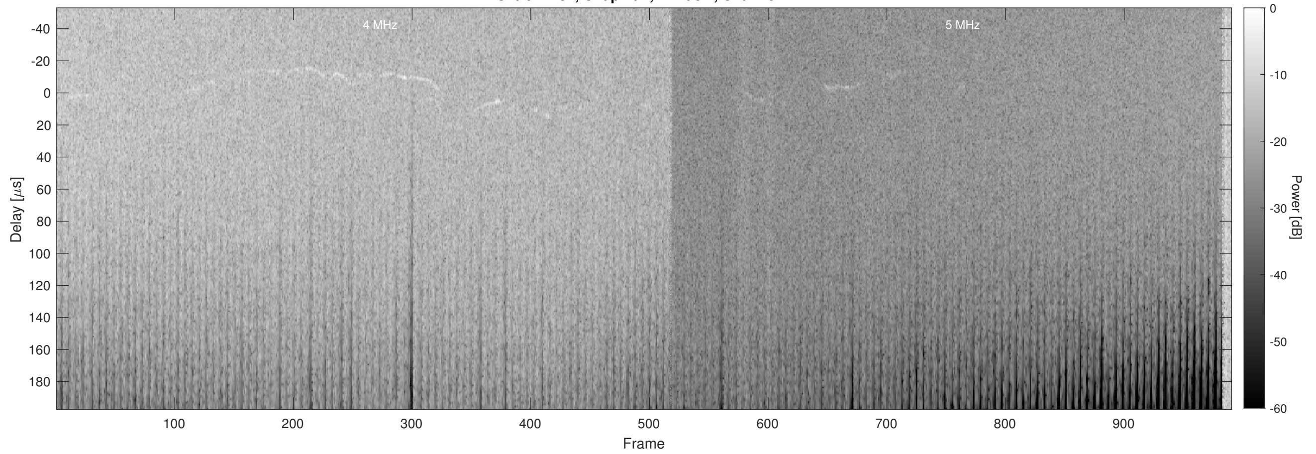
Orbit 12731, Chapman, Window, Channel 2
