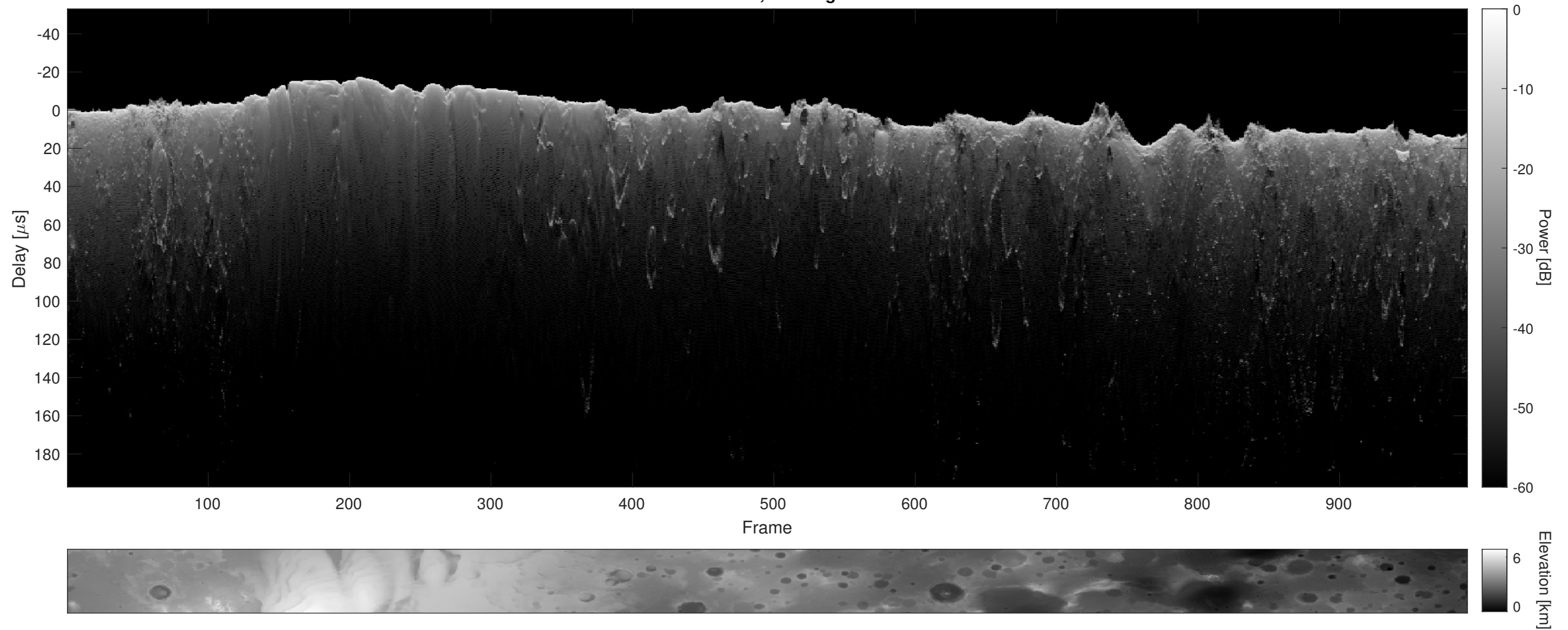
Orbit 12731, Cluttergram
