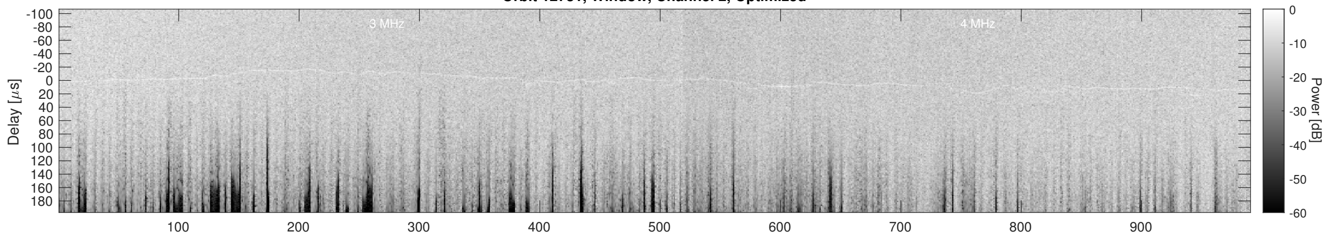
Orbit 12731, Cluttergram
