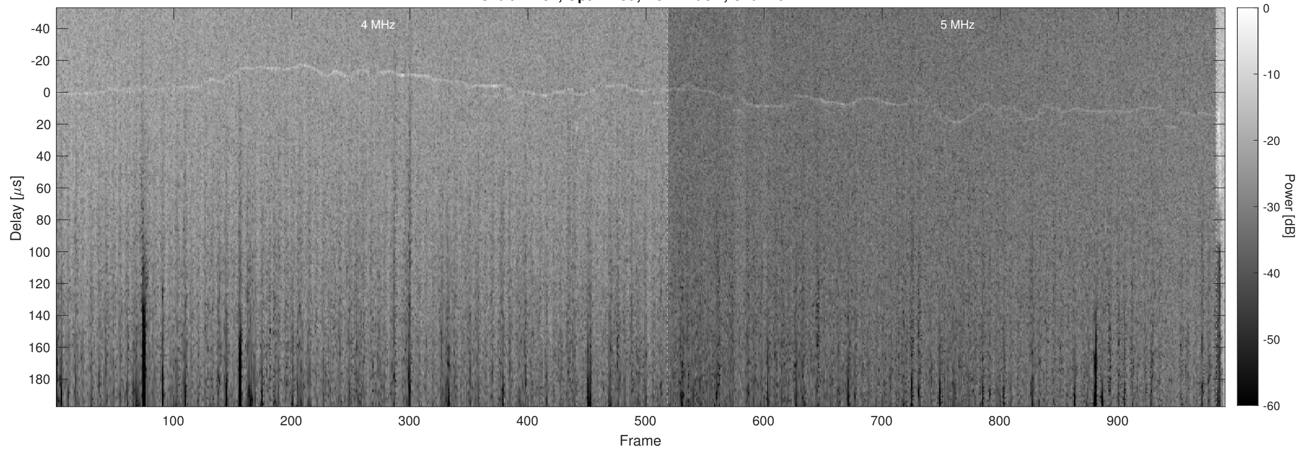
Orbit 12731, Optimized, No Window, Channel 2
