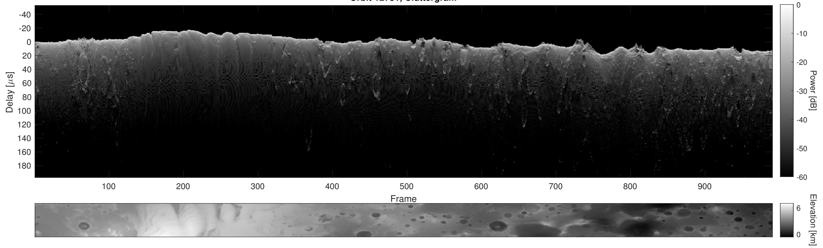
Orbit 12731, Cluttergram
