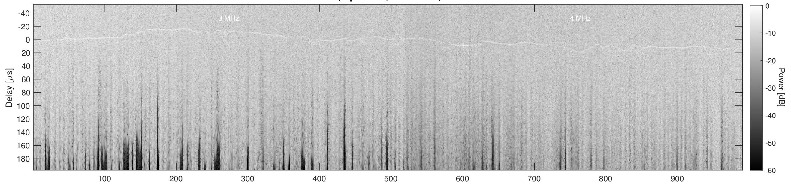
Orbit 12731, Cluttergram
